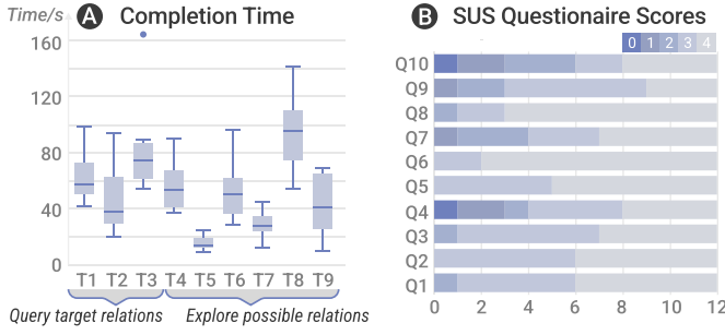
Fig. 13. The quantitative results of our task-based user study. (A) The record of completion time reveals a high task pass rate and varied difficulty. (B) We summarized the distribution of SUS scores given by subjects. In general, subjects commented positively on the usability of RelaQ.
