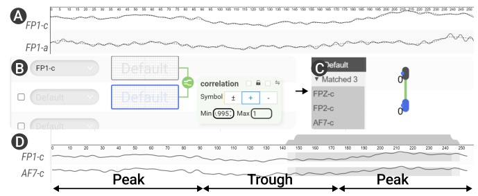
Fig. 11. This displays Q1 and R1 for the first case. (A) The time series of Fp1-c and -a. (B) Query time series correlated to Fp1-c. (C) Results include Fp2-c, Fpz-c, and AF7-c. (D) Results mainly distribute in the second peak.
