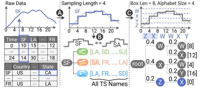
Fig. 5. This shows a three-step data preprocessing method using an example. The raw data contains multiple time series ( SF , LA , ..., FR ) and label descriptions ( SF 's State being CA ). (A) First, time series are compressed by taking the average of segments with Sampling Length=4 so the blue line shows compressed data. (B) Second, relation indexes are computed. We compute the relation strength between each pair of time series and record all time series names in the descending order of relation strength on the whole length. e.g., SA is the city with the highest similarity strength with SF . (C) Third, trend indexes are computed. We transformed compressed data into symbolic sequences using SAX [27] (alphabet size = 4). The sequence ( ZXWXY ) is built as a trie (depth = 8/4 = 2 , box length = 8, sampling length = 4). e.g., The starting points of ZX contain [0], and the ratio is 0.2.
