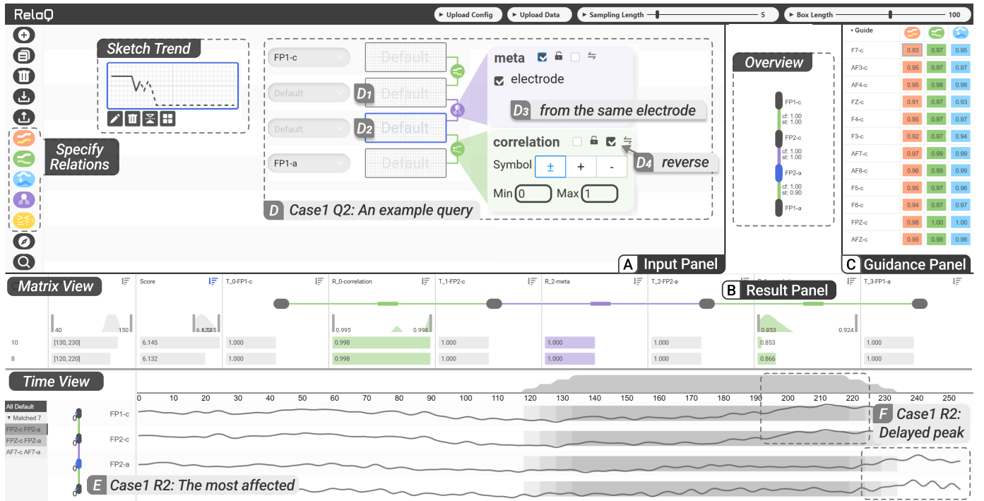
Fig. 2. The user interface of RelaQ. It is composed of three main parts: In the (A) input panel, users can sketch trends and specify relations. In the (B) result panel, users can obtain an overview, compare results in the matrix view, and inspect details in the time view. In the (C) guidance panel, there are recommended timeboxes. Besides, this figure also displays part of the first case in Sec. V-A: (D) an example query and (E-F) some patterns in its results.
