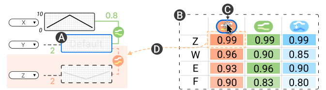
Fig. 10. The guidance panel's design. (A) The focus timebox. (B) The recommended timeboxes that can be added to the query. (C) The relation icon that can be clicked to sort recommendations. (D) The preview of a new query after hovering.
