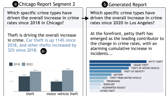
Figure 5: The process of generating the second segment.
